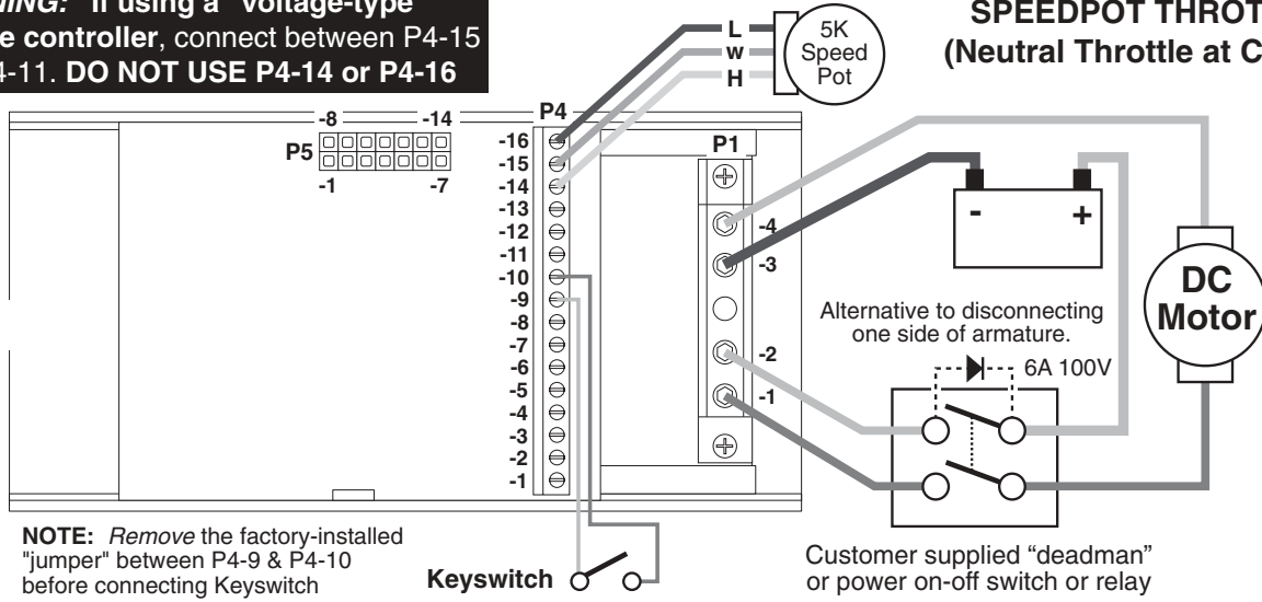
Basic Connections for "Wig-Wag" operation with "SpeedPot" input
