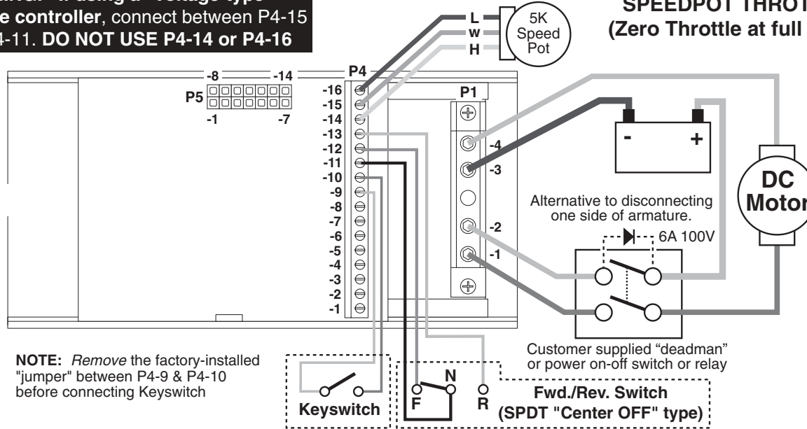
As above except "Single Direction" operation (using Direction Switch)
