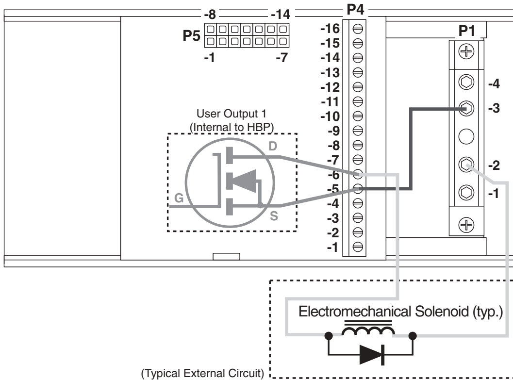
User Output 1 Typical Connections
