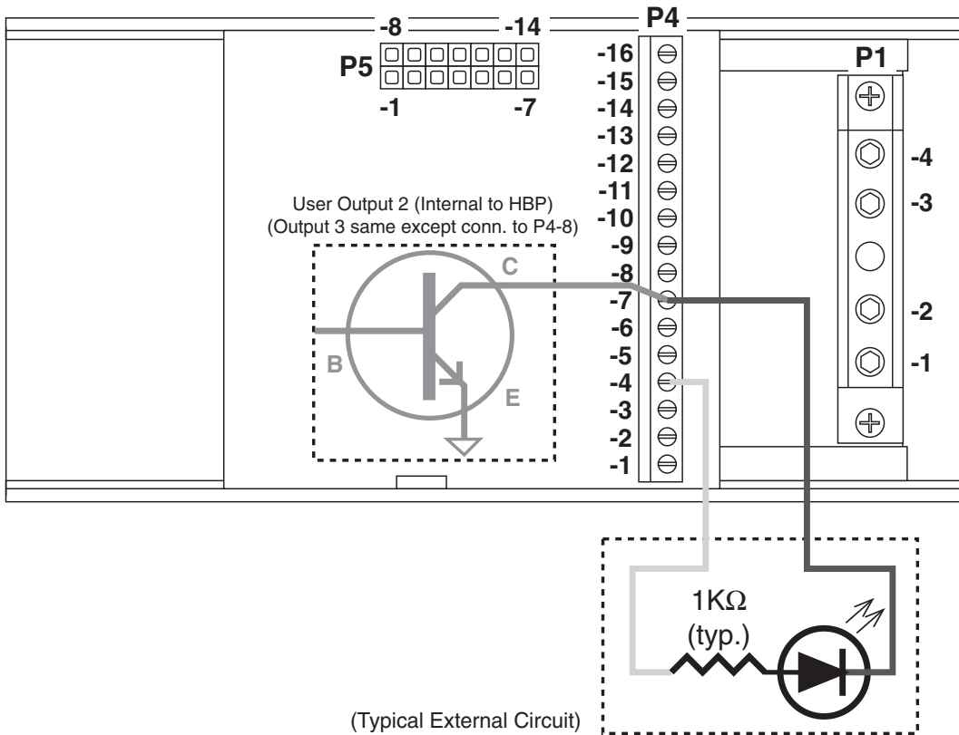
User Output 2 & 3 Typical Connections
